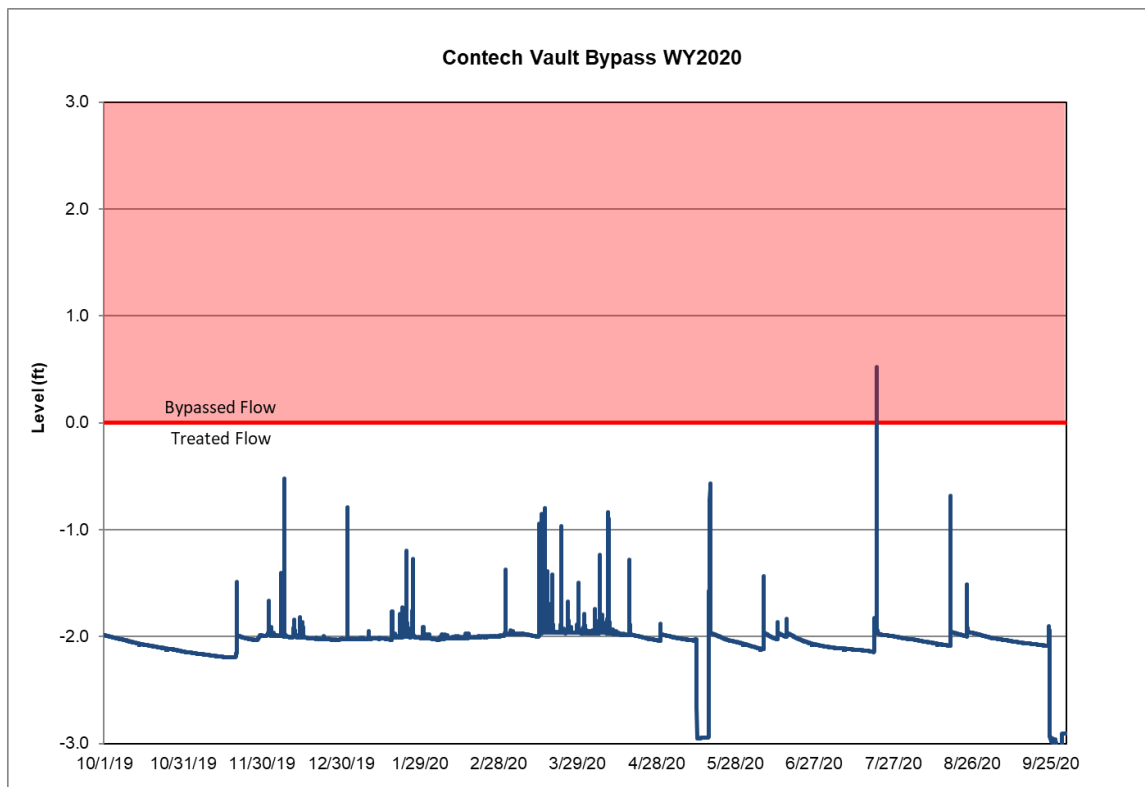
Figure 1: Bypassed flow in the Contech MFS vault for WY20 to date.
