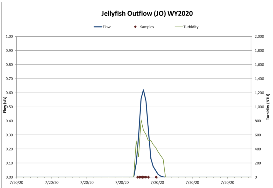
Figure 8: Hydrograph, continuous turbidity and sample distribution at the Jellyfish Outflow for the 7/20/20 thunderstorm event.
