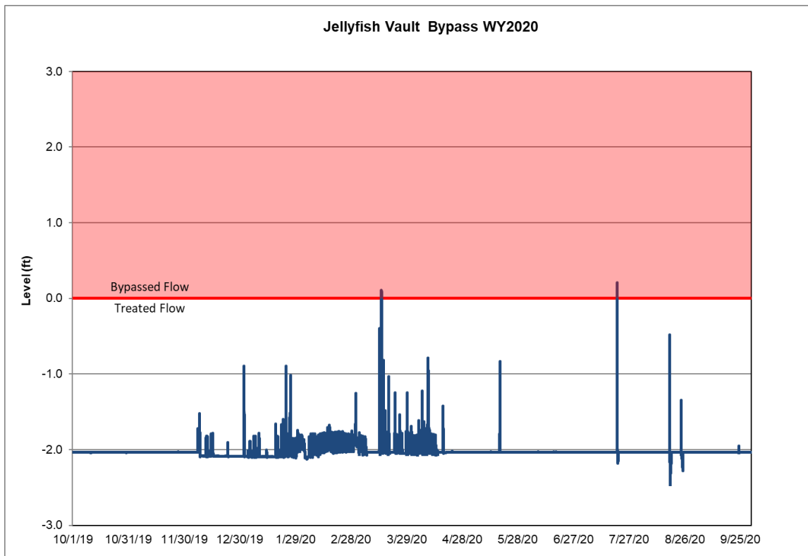
Figure 2: Bypassed flow in the Jellyfish vault for WY20 to date.
