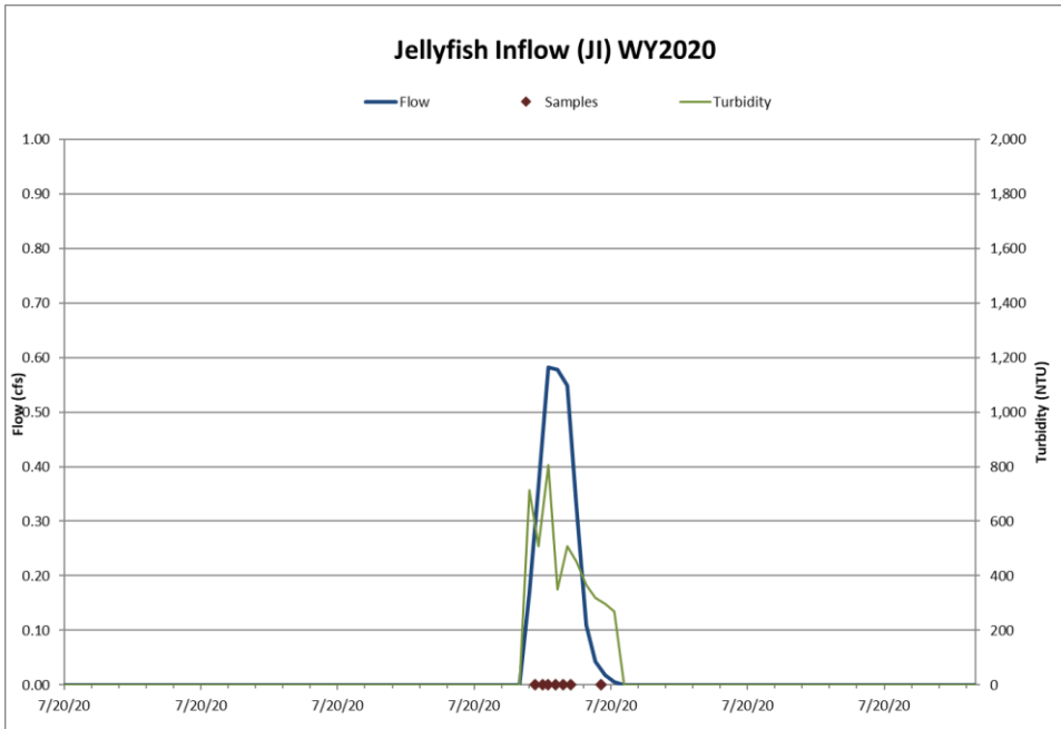
Figure 7: Hydrograph, continuous turbidity and sample distribution at the Jellyfish Inflow for the 7/20/20 thunderstorm event.
