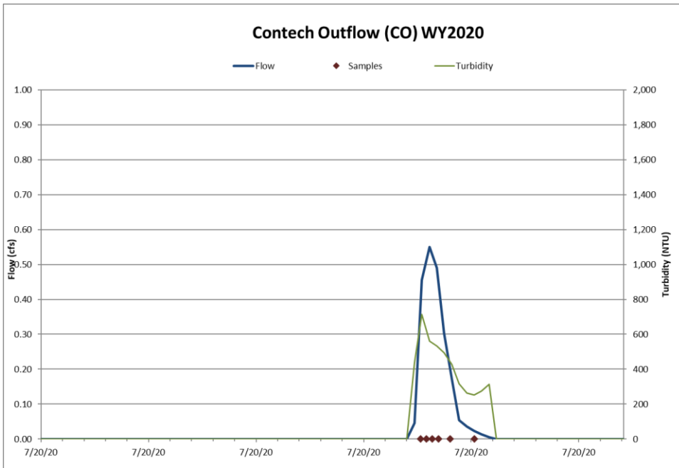
Figure 9: Hydrograph, continuous turbidity and sample distribution at the Contech Outflow for the 7/20/20 thunderstorm event. (Jellyfish Inflow data substituted for Contech Inflow data for this event.)
