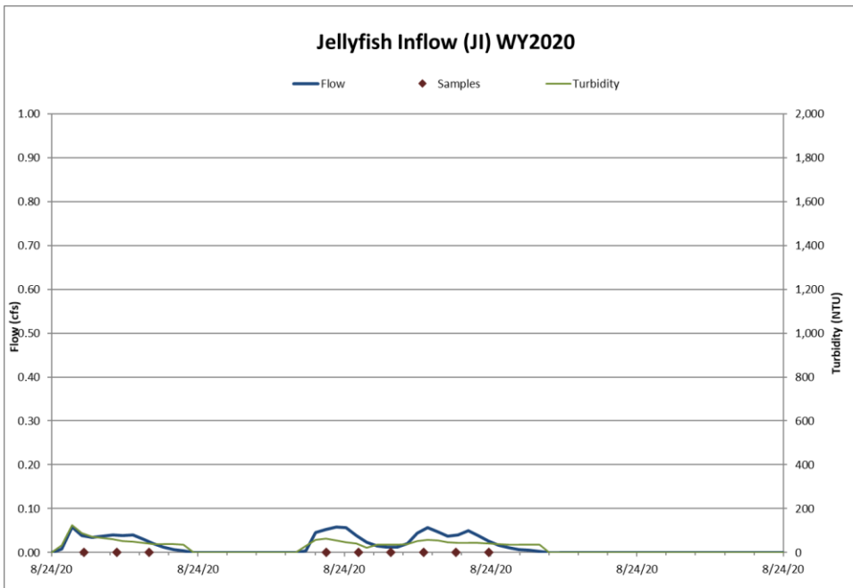
Figure 10: Hydrograph, continuous turbidity and sample distribution at the Jellyfish Inflow for the 8/24/20 thunderstorm event.
