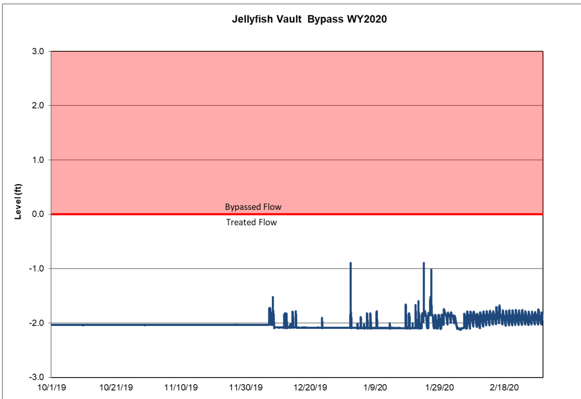
Figure 2: No bypassed flow in the Jellyfish vault for WY20 to date.
