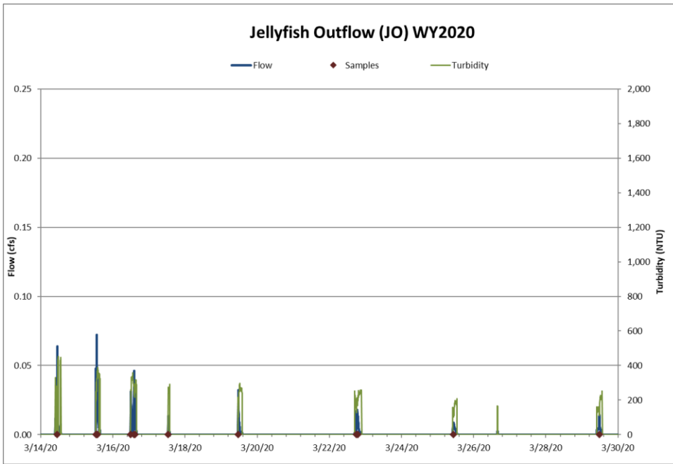
Figure 9: Hydrograph, continuous turbidity and sample distribution at the Jellyfish Outflow for the 3/14/20 - 3/29/20 snowmelt event.
