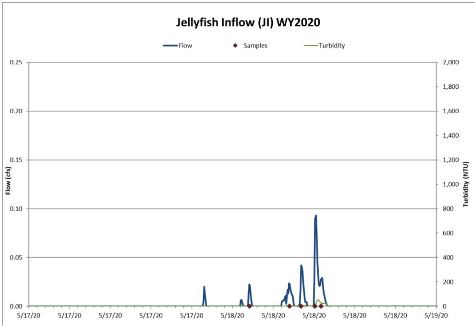
Figure 10: Hydrograph, continuous turbidity and sample distribution at the Jellyfish Inflow for the 5/17/20 - 5/18/20 rain event.
