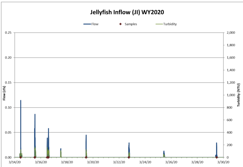
Figure 8: Hydrograph, continuous turbidity and sample distribution at the Jellyfish Inflow for the 3/14/20 - 3/29/20 snowmelt event.
