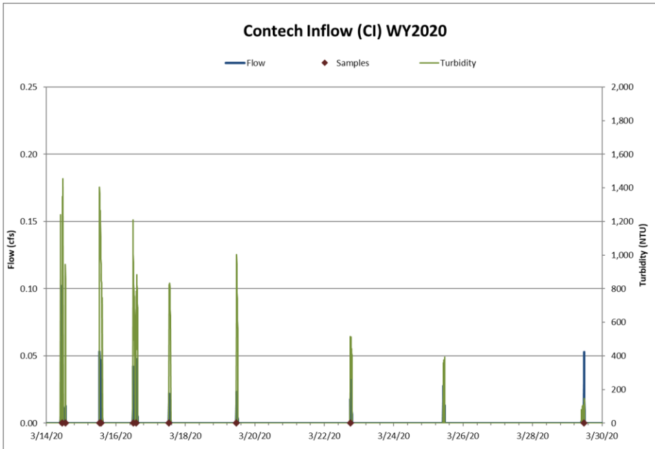
Figure 7: Hydrograph, continuous turbidity and sample distribution at the Contech MFS Inflow for the 3/14/20 - 3/29/20 snowmelt event.
