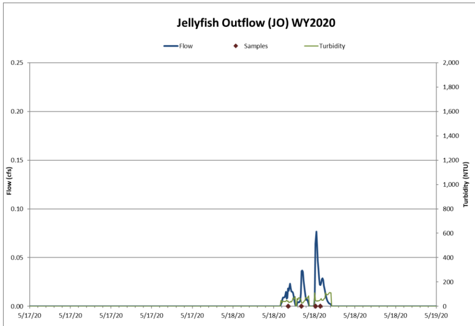
Figure 11: Hydrograph, continuous turbidity and sample distribution at the Jellyfish Outflow for the 5/17/20 - 5/18/20 rain event.
