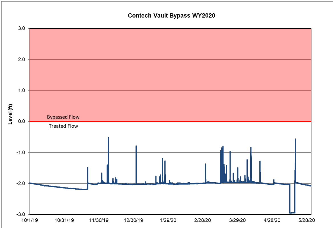
Figure 1: No bypassed flow in the Contech MFS vault for WY20 to date.
