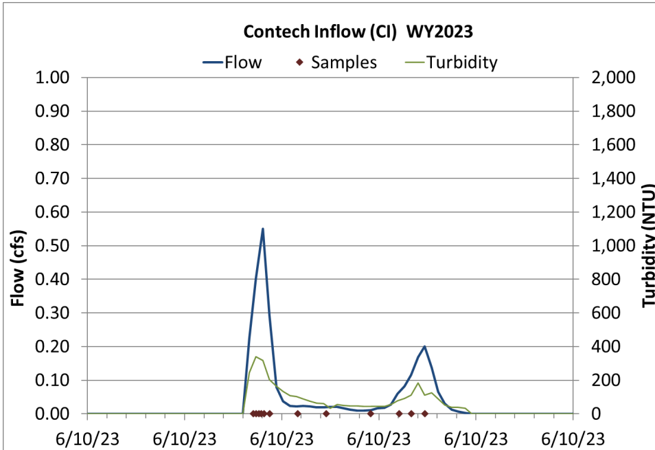
Figure 11 Hydrograph, continuous turbidity, and sample distribution at the Contech Inflow for the 6/10/2023 thunderstorm event.
