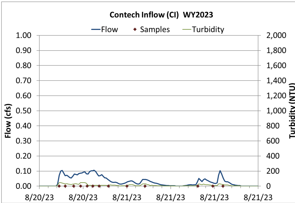
Figure 19 Hydrograph, continuous turbidity, and sample distribution at the Contech Inflow for the 8/20/23-8/21/23 rain event.
