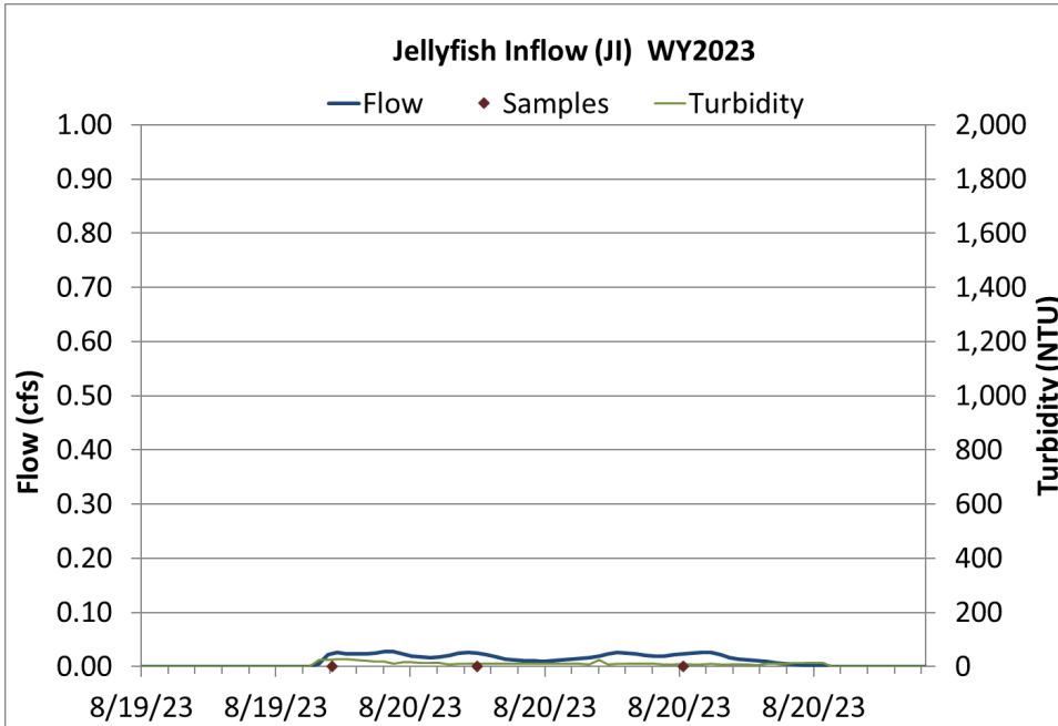
Figure 17 Hydrograph, continuous turbidity, and sample distribution at the Jellyfish Inflow for the 8/19/23-8/20/23 thunderstorm event.
