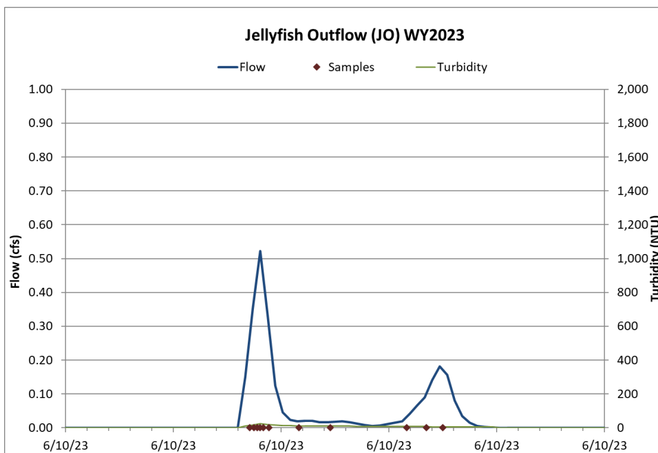
Figure 14 Hydrograph continuous turbidity, and sample distribution at the Jellyfish Outflow for the 6/10/2023 thunderstorm event.
