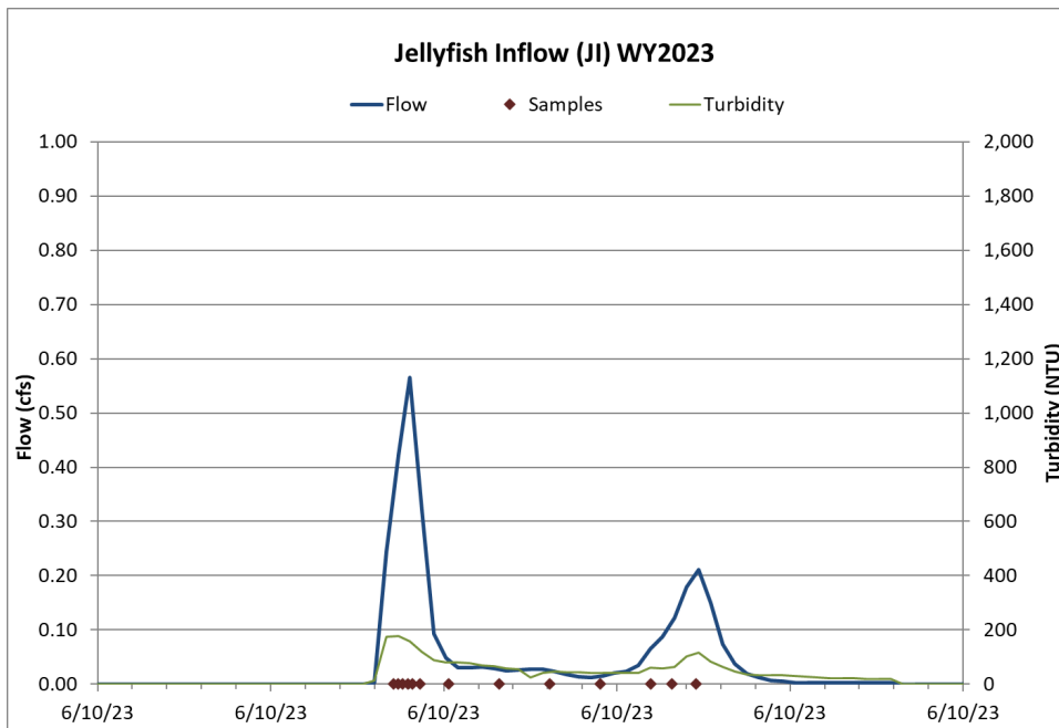
Figure 13 Hydrograph, continuous turbidity, and sample distribution at the Jellyfish Inflow for the 6/10/2023 thunderstorm event.
