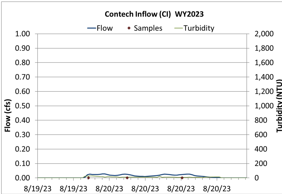
Figure 15 Hydrograph, continuous turbidity, and sample distribution at the Contech Inflow for the 8/19/23-8/20/23 thunderstorm event.
