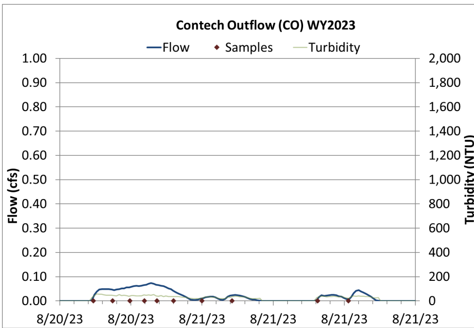
Figure 20 Hydrograph, continuous turbidity, and sample distribution at the Contech Outflow for the 8/20/23-8/21/23 rain event.
