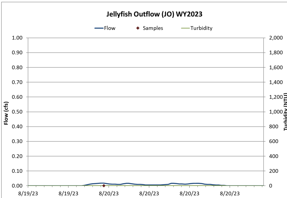
Figure 18 Hydrograph, continuous turbidity, and sample distribution at the Jellyfish Outflow for the 8/19/23-8/20/23 thunderstorm event.
