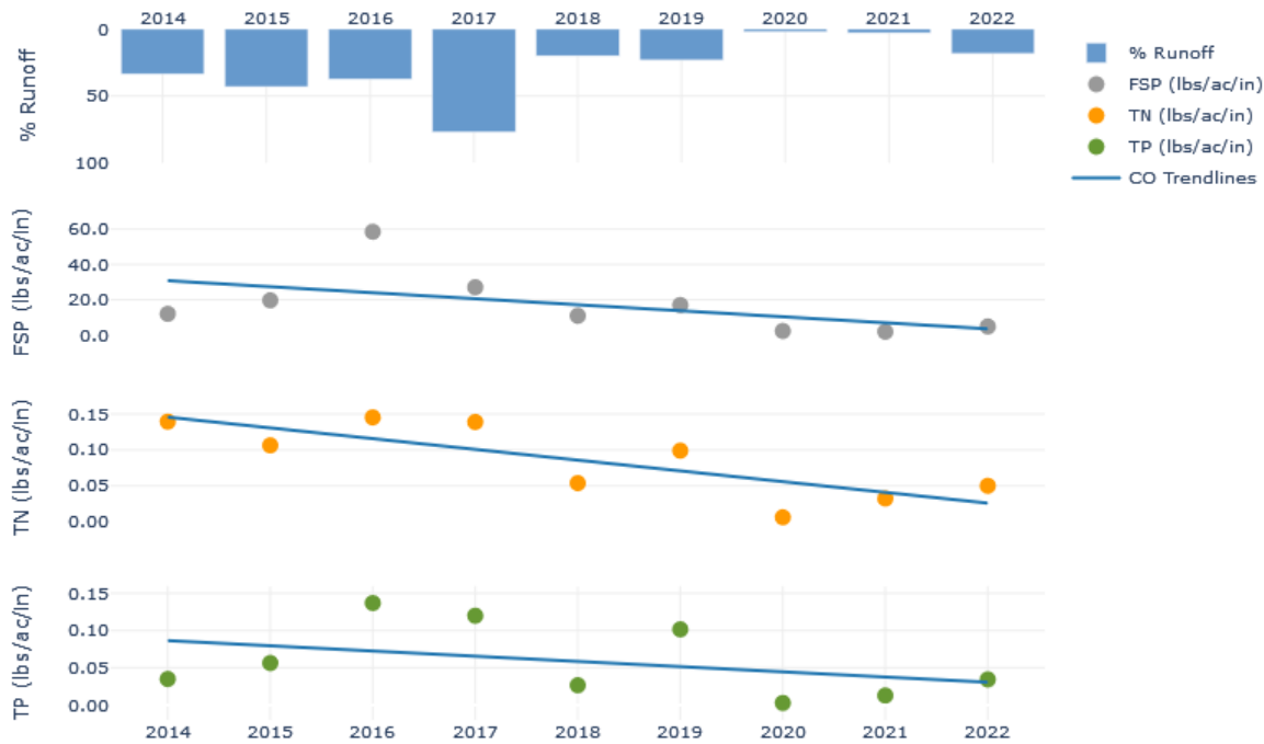
Figure 8 9-year rainfall normalized annual pollutant load trends in FSP, TN, and TP loads at the Contech MFS Outflow, WY14-22.
