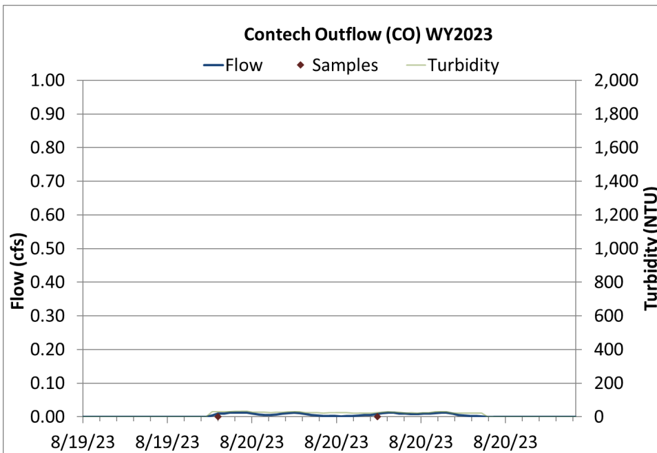
Figure 16 Hydrograph, continuous turbidity, and sample distribution at the Contech Outflow for the 8/19/23-8/20/23 thunderstorm event.
