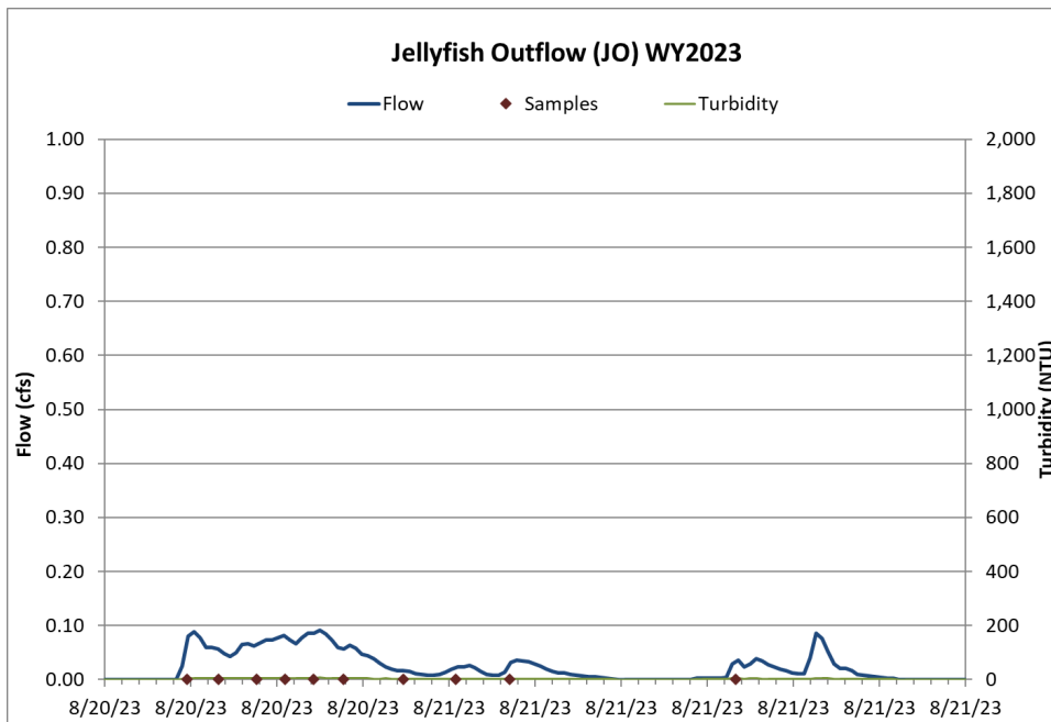
Figure 22 Hydrograph, continuous turbidity, and sample distribution at the Jellyfish Outflow for the 8/20/23-8/21/23 rain event.
