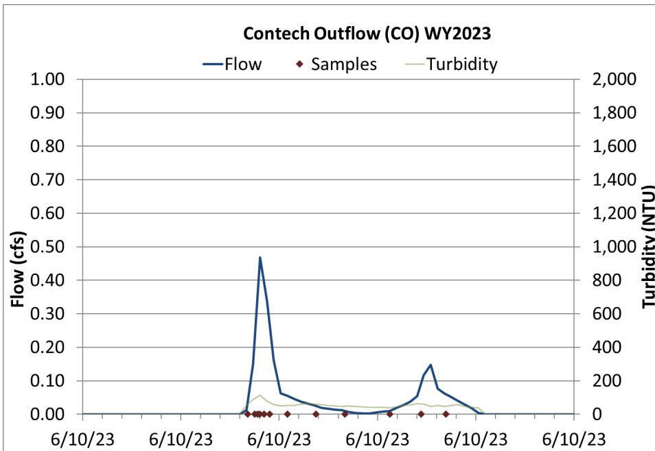
Figure 12 Hydrograph, continuous turbidity, and sample distribution at the Contech Outflow for the 6/10/2023 thunderstorm event.
