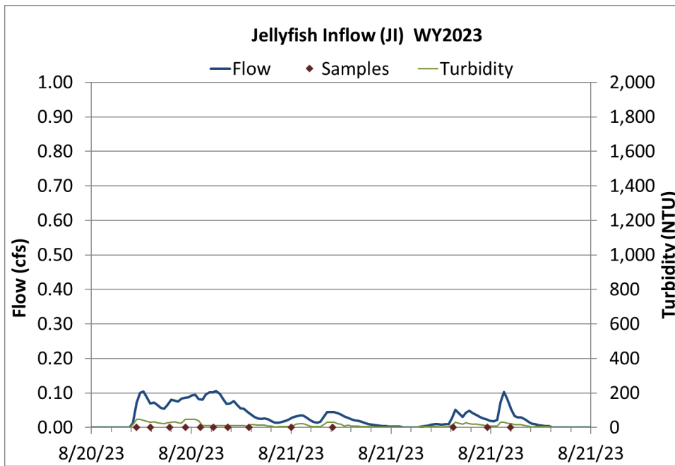
Figure 21 Hydrograph, continuous turbidity, and sample distribution at the Jellyfish Inflow for the 8/20/23-8/21/23 rain event.
