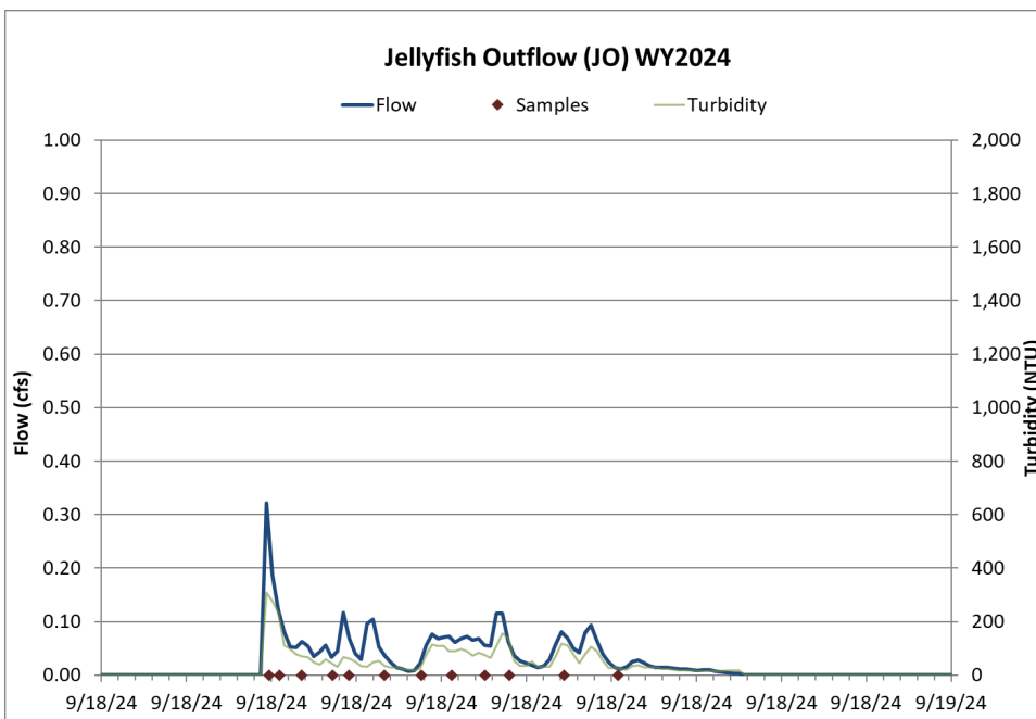
Figure 11 Hydrograph, continuous turbidity, and sample distribution at the Jellyfish Outflow for the 9/18/2024 thunderstorm event.
