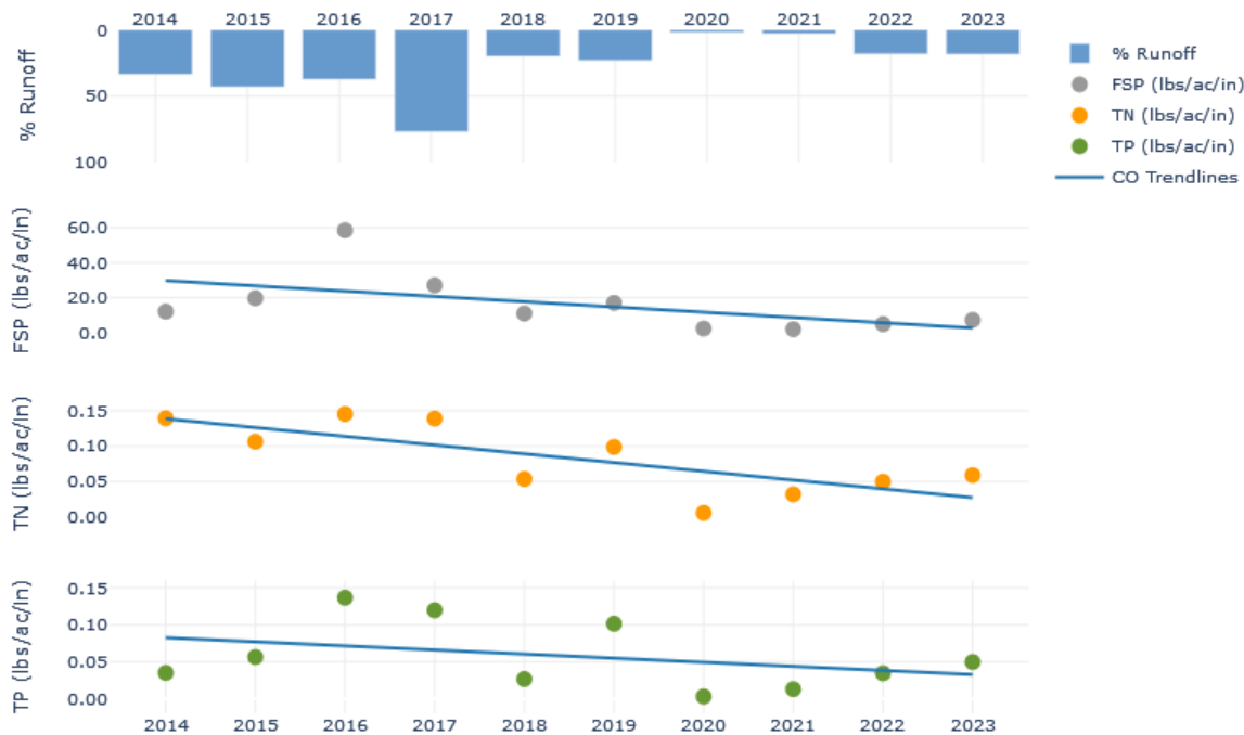
Figure 5 10-year rainfall normalized annual pollutant load trends in FSP, TN, and TP loads at the Contech MFS Outflow, WY14-23.
