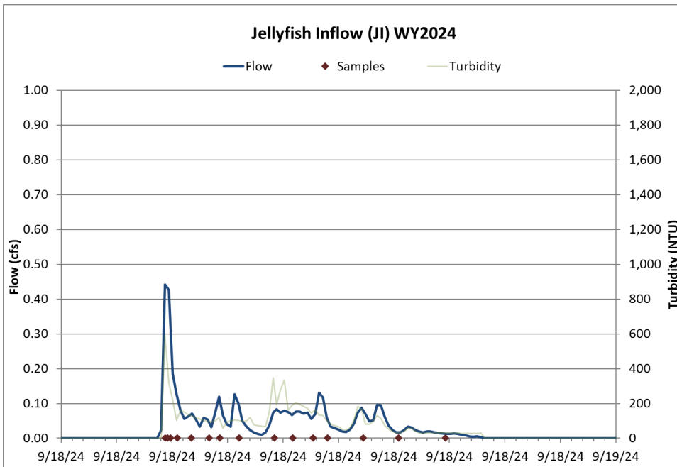
Figure 10 Hydrograph, continuous turbidity, and sample distribution at the Jellyfish Inflow for the 9/18/2024 thunderstorm event.
