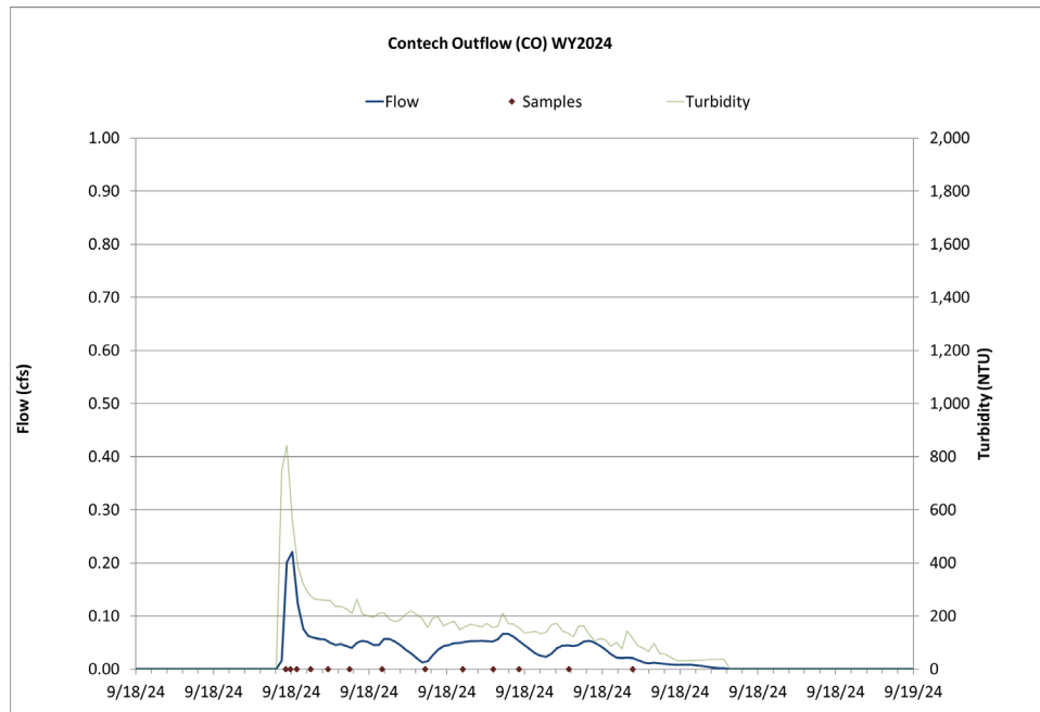
Figure 9 Hydrograph, continuous turbidity, and sample distribution at the Contech Outflow for the 9/18/2024 thunderstorm event.
