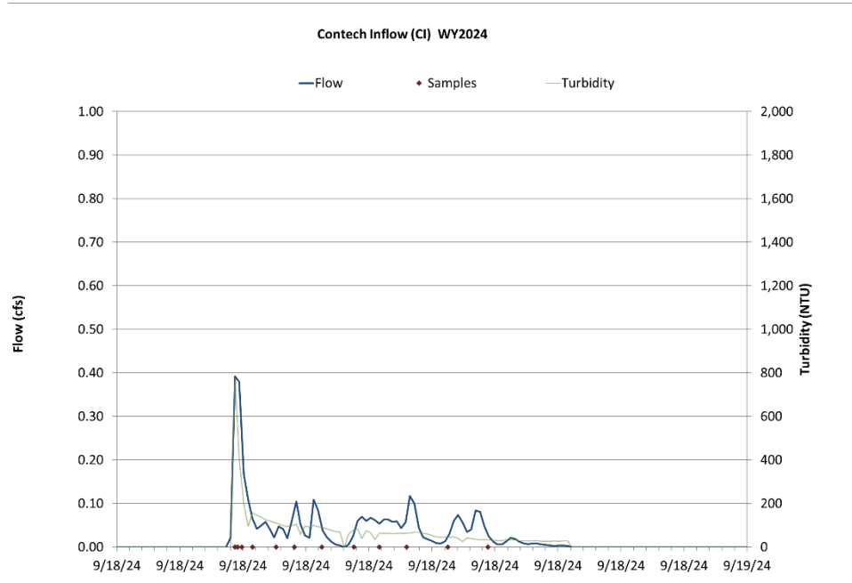
Figure 8 Hydrograph, continuous turbidity, and sample distribution at the Contech Inflow for the 9/18/2024 thunderstorm event.
